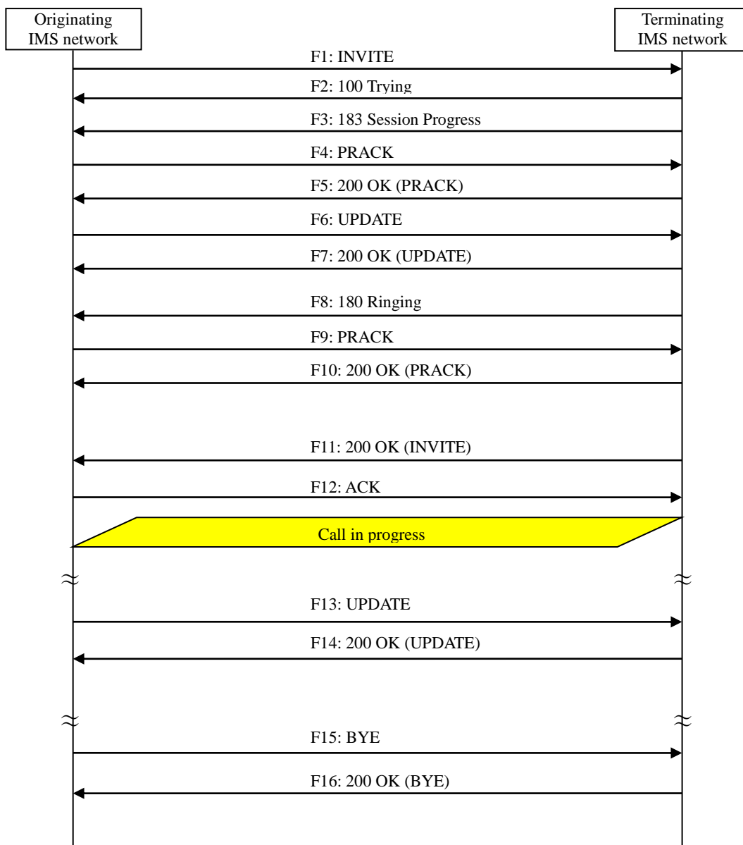
Appendix Figure vii.2.1.2.1-1 / JJ-90.30: Basic call (Call is released by originating side) < Originating from mobile IMS network and terminating in mobile IMS network (Initial condition: resources of both originating and terminating side are not reserved)>
