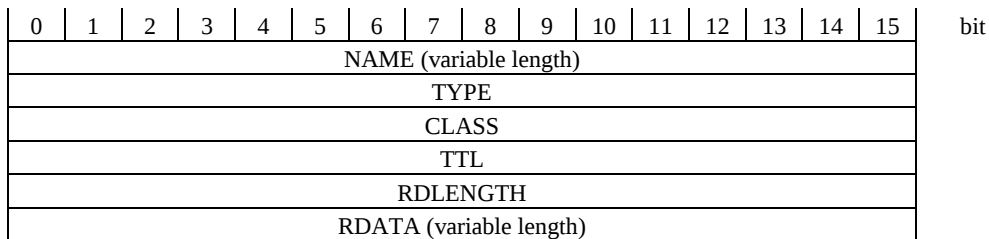
Figure 4.3.1.3-1 / JJ-90.31: Format of the resource records
