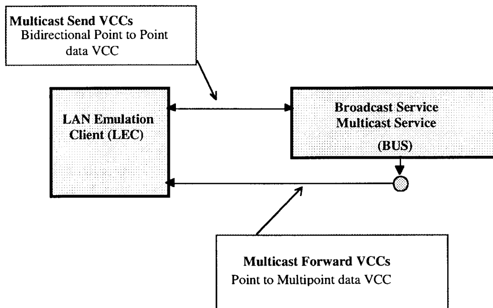
Figure 7. LAN Emulation Client Broadcast/Multicast Connections
