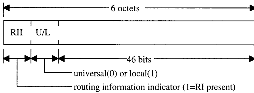
Figure 17. Source Address Field
