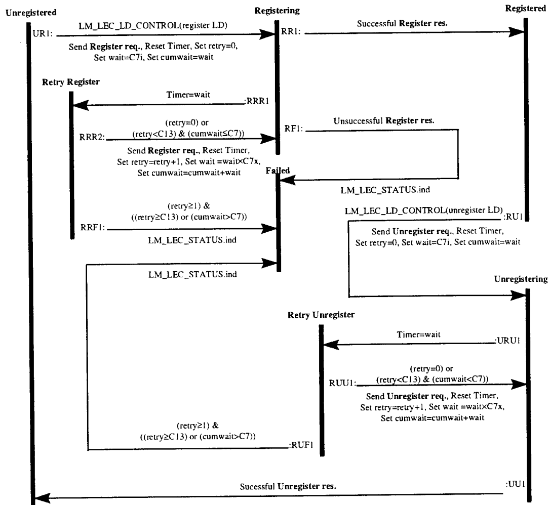
Figure 13. Registration State Machines
