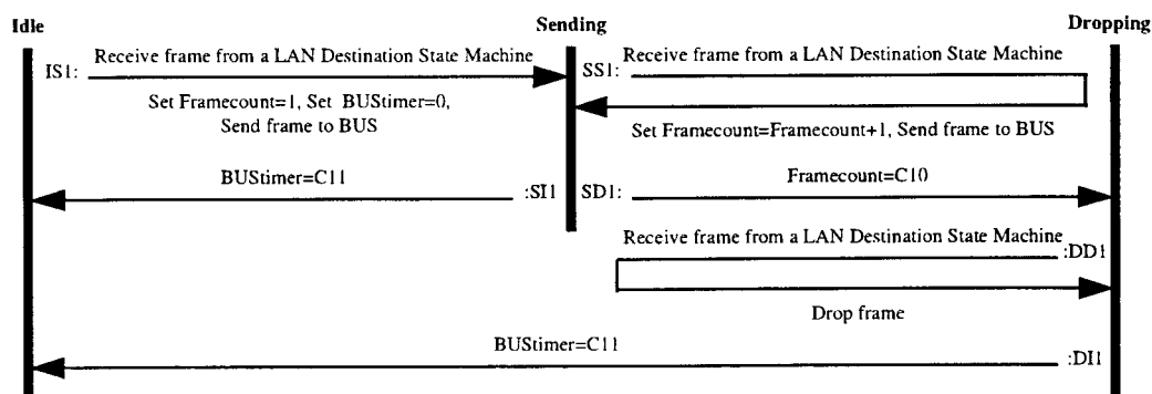
Figure 16. LAN Destination Unconnected State Machine
