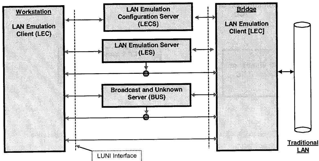
Figure 3. Example of LAN Emulation Client Flows across LUNI
