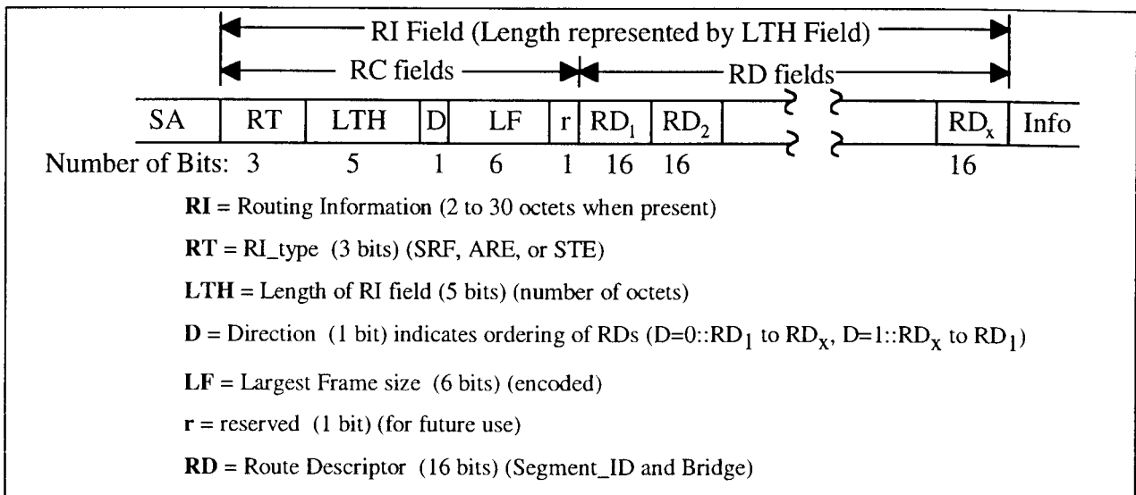
Figure 18. Routing Information Field Content
