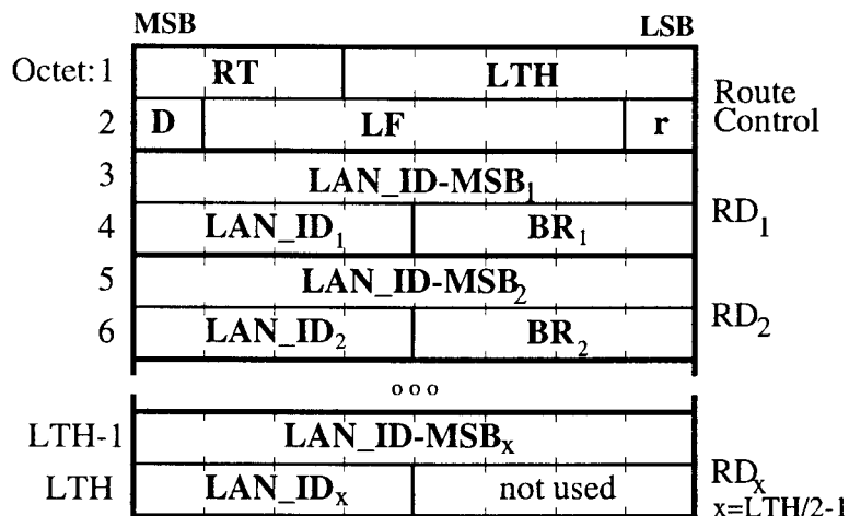
Figure 19. Routing Information Field Format
