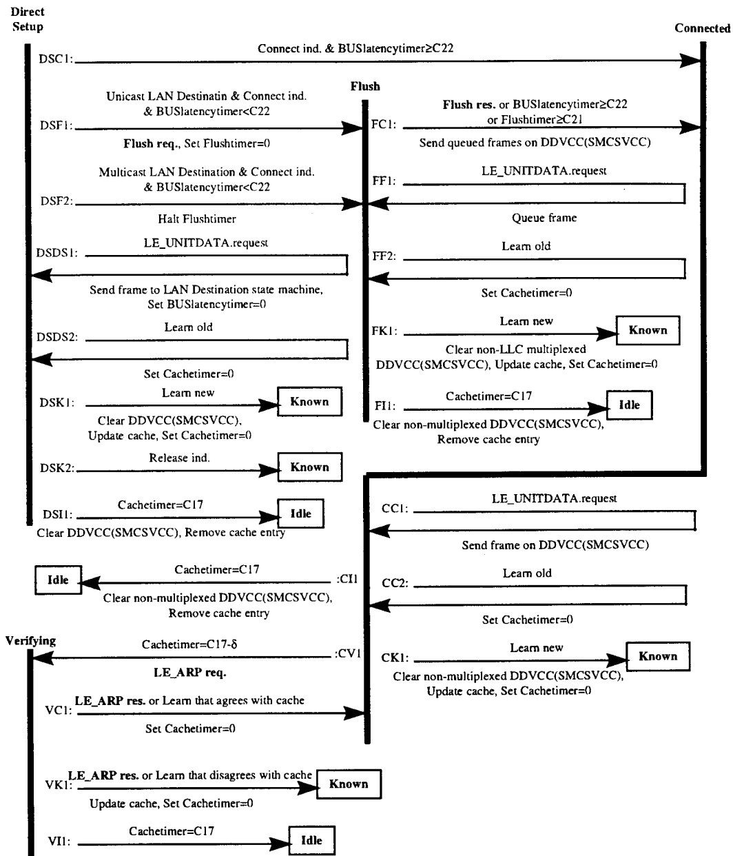
Figure 15. LAN Destination State Machine (Part 2)
