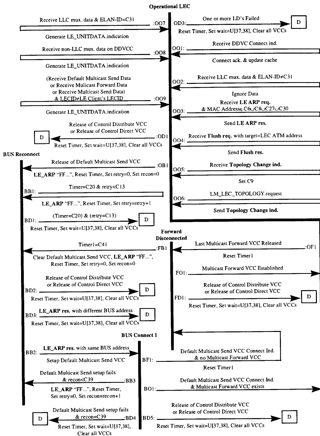
Figure 12. LE Client State Machine (Operational)
