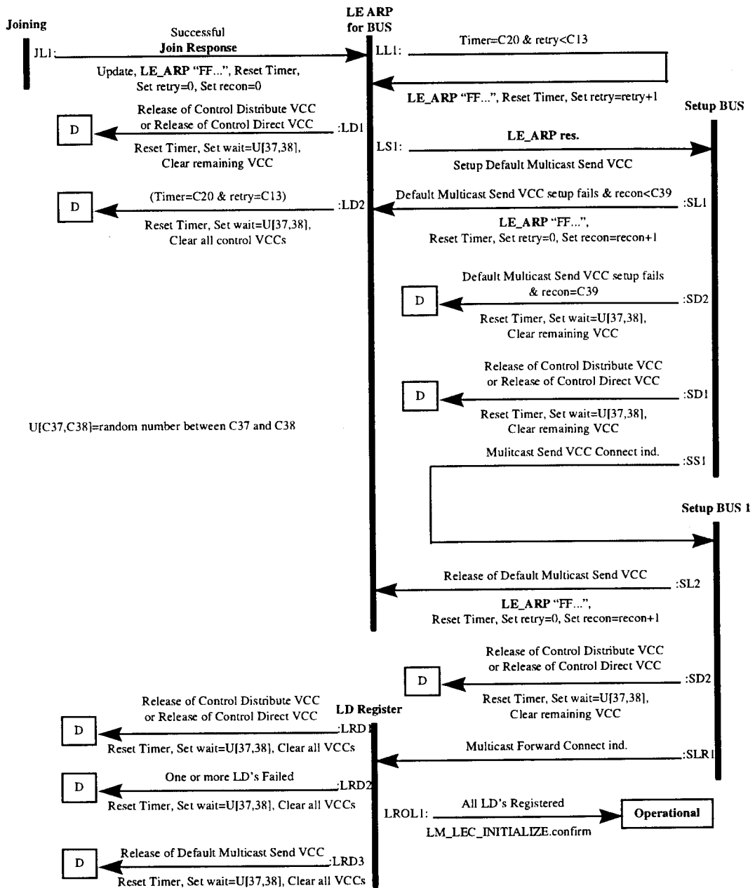
Figure 11. LE Client State Machine (Join, LE_ARP)
