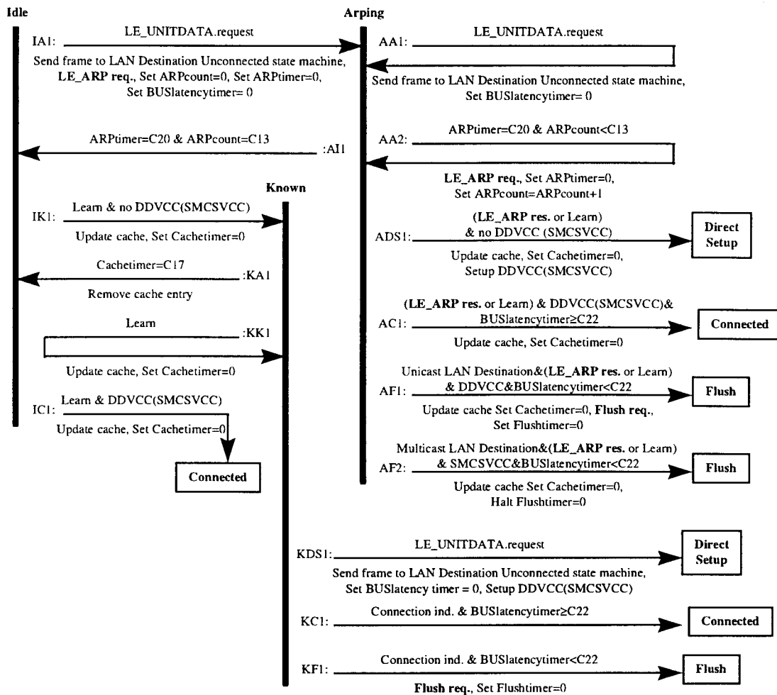
Figure 14. LAN Destination State Machines (Part 1)
