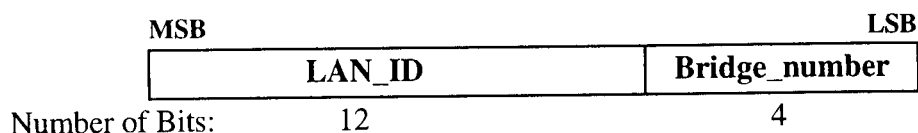
Figure 20. Route Descriptor Format
