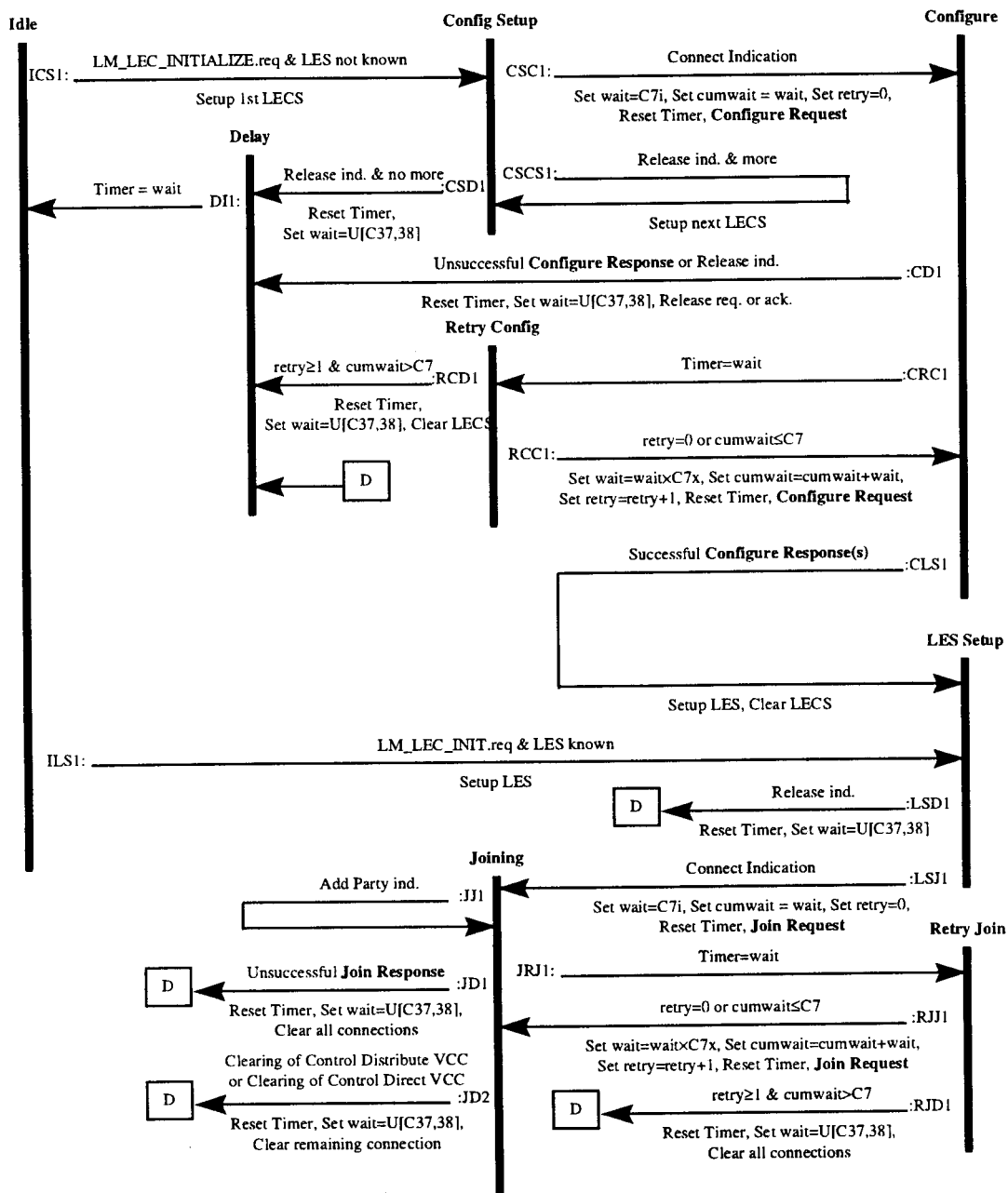
Figure 10. LE Client State Machine (Initialization)
