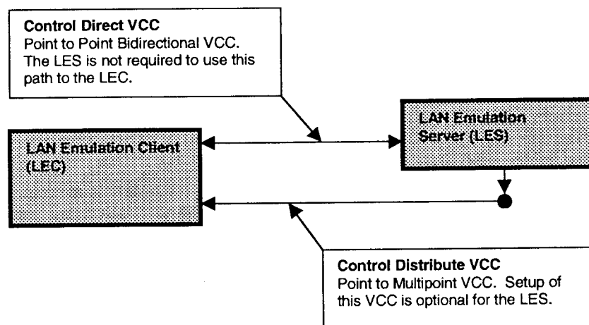
Figure 5. LAN Emulation Client to LAN Emulation Server (LES) Control Connections
