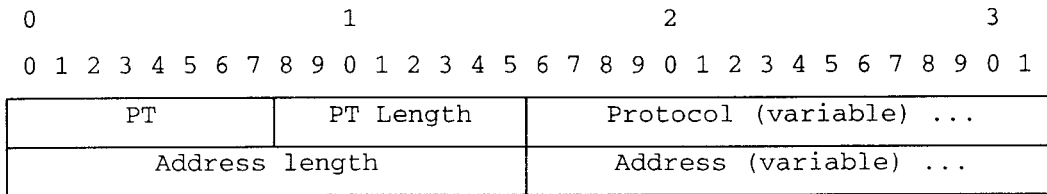
Figure 22. ISO 10747 Address Format
