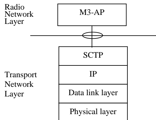
Figure 5.1.1: M3 signalling bearer protocol stack
